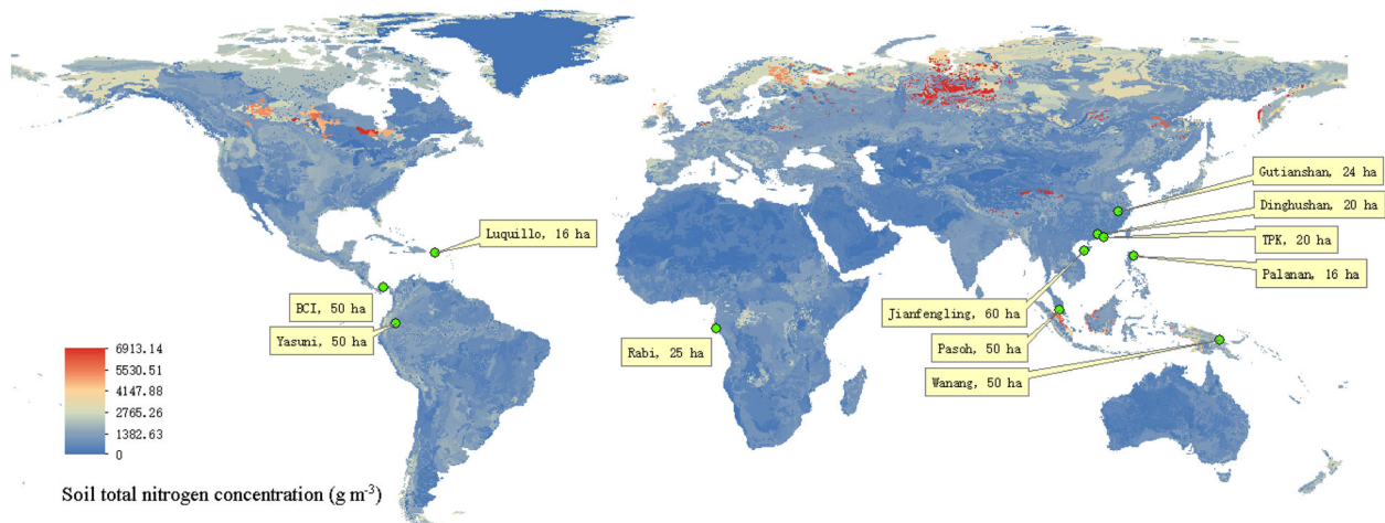
Fig. 1 Global map showing the location of the 11 Forest-GEO plots. This map is overlaid with the IGBP-DIS 1-m depth soil total N concentration (5 × 5 arc-minute resolution) 42 .
